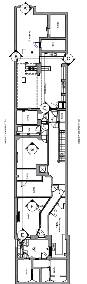
00 Key plan Basement NTS
