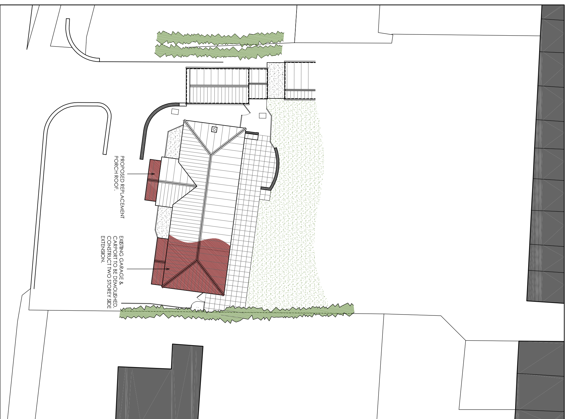
BLOCK & ROOF PLAN 1:200
