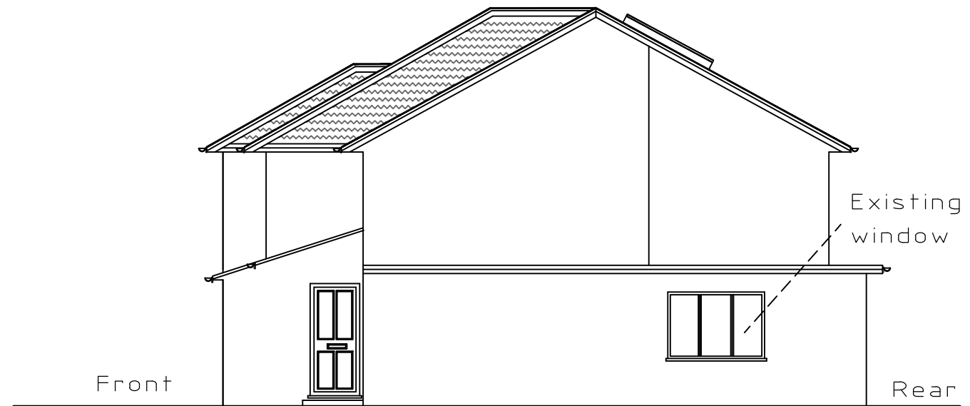
Proposed Side Elevation Looking From No: 292
