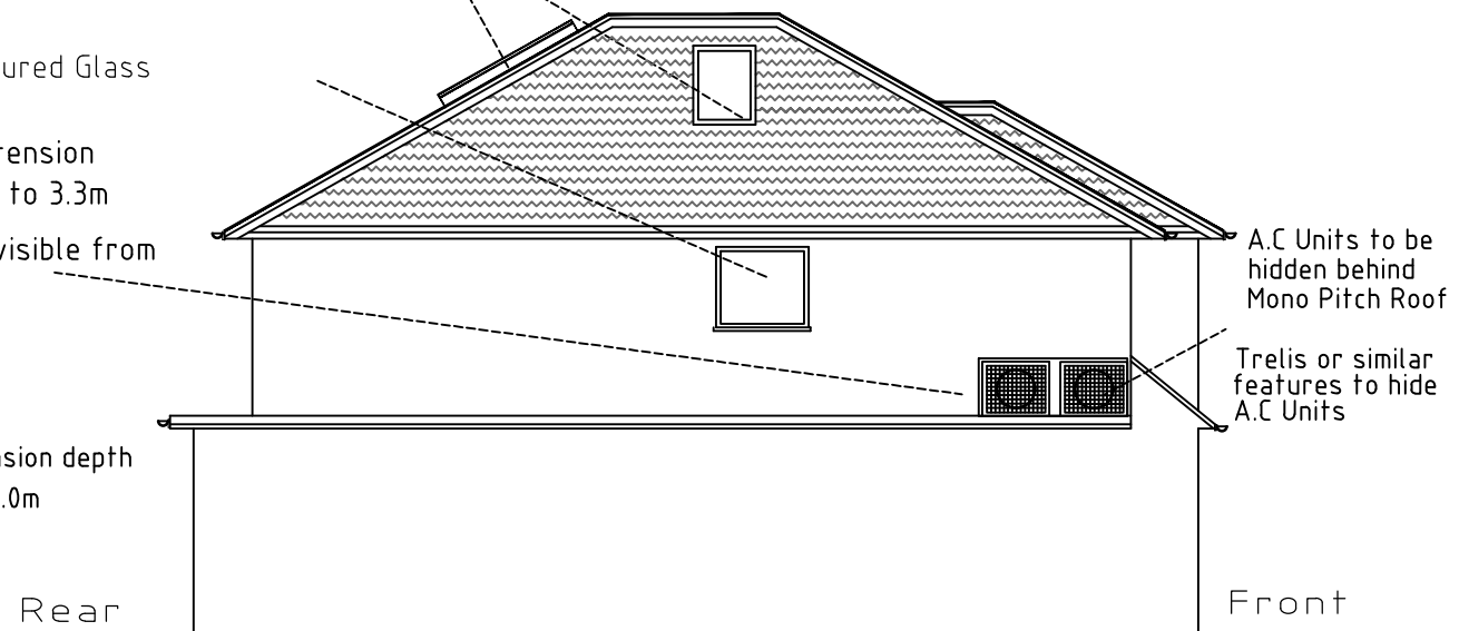
Proposed Side Elevation Looking From No: 296
