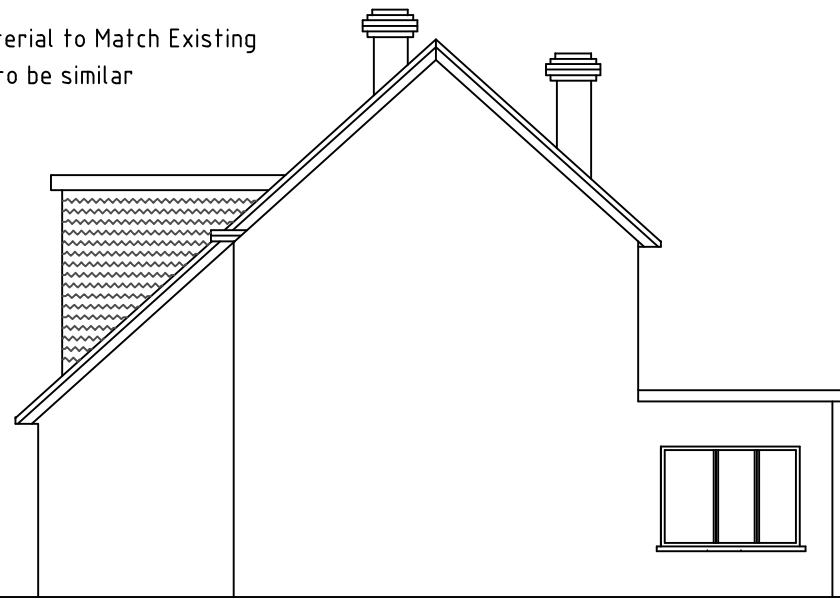
Existing Side Elevation Looking From No: 292
