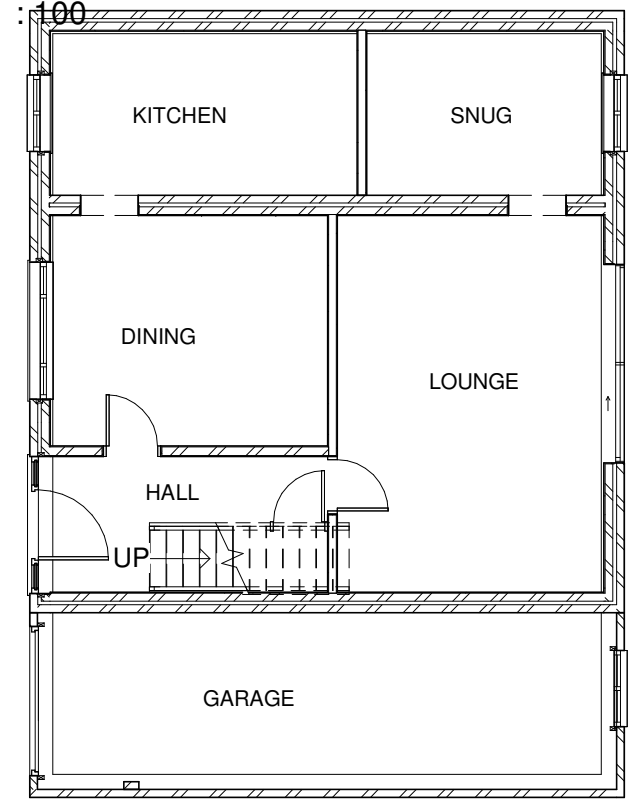
3 Proposed Ground Floor 1 : 100
