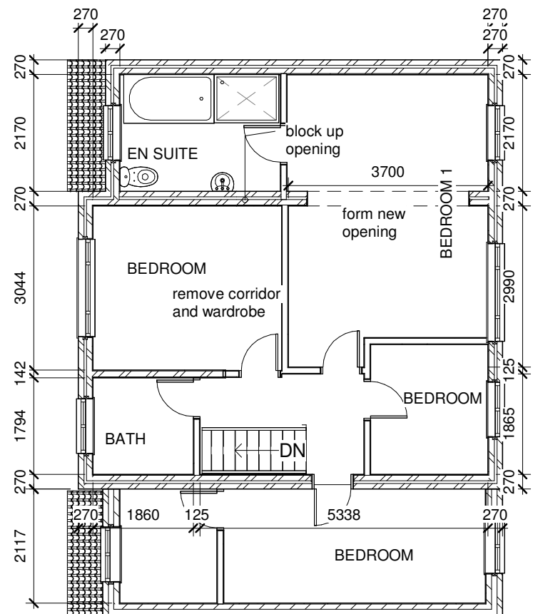
4 Proposed First Floor 1 : 100
