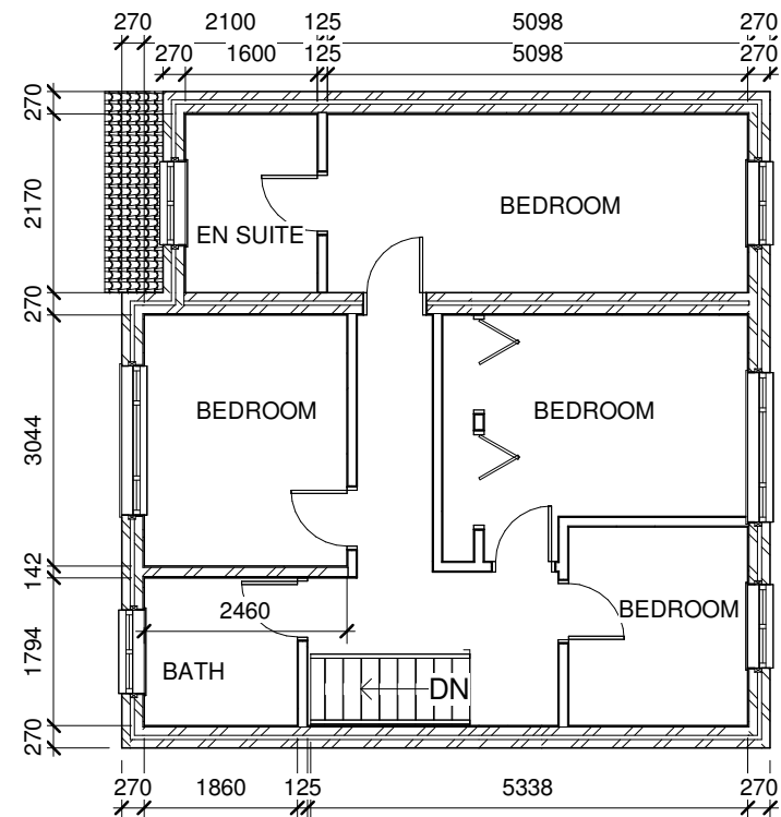
2 Existing First Floor 1 : 100
