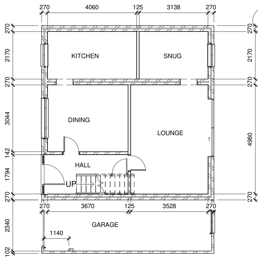
1 Existing Ground Floor 1 : 100
