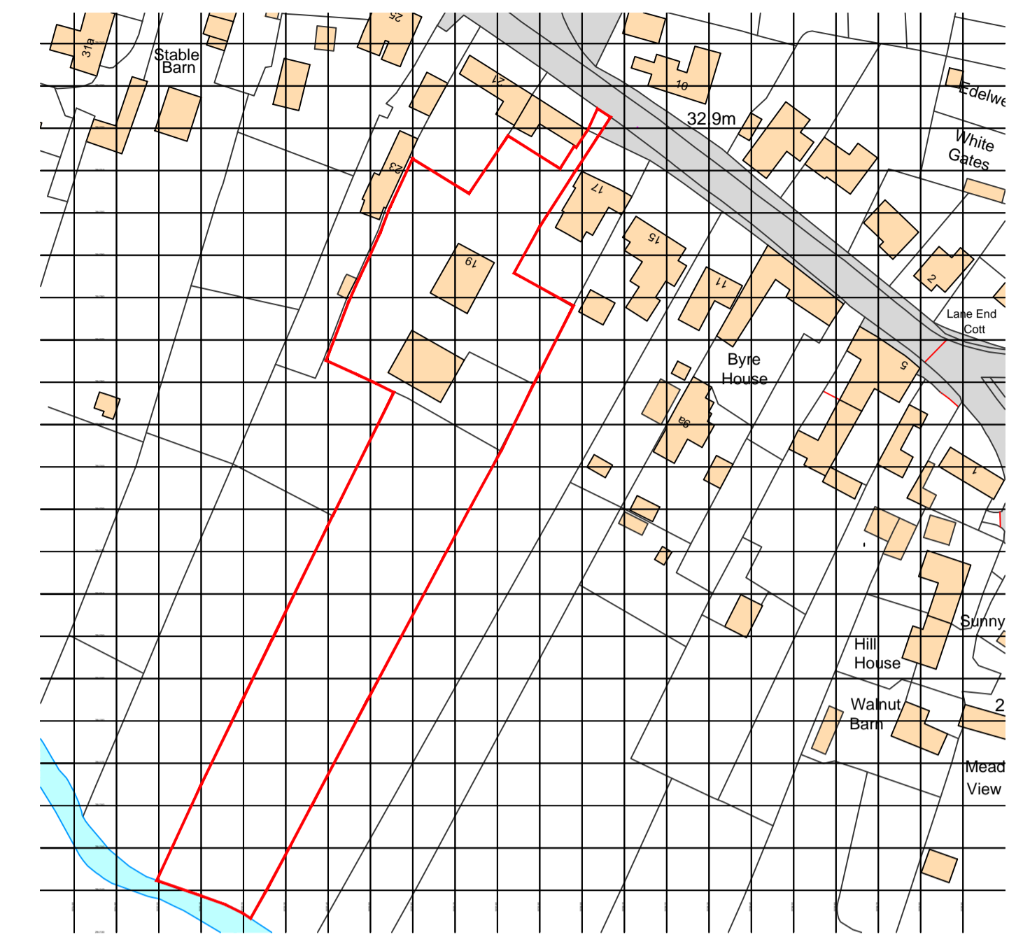
A-100 1 SITE LOCATION PLAN
