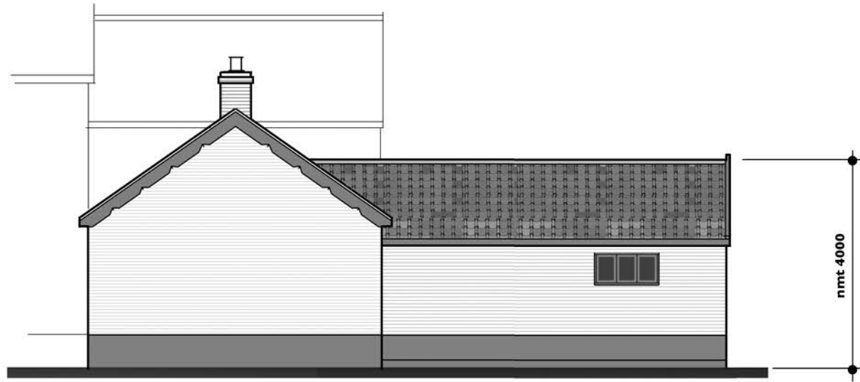
:: East :: Proposed :: 1:100 ::
