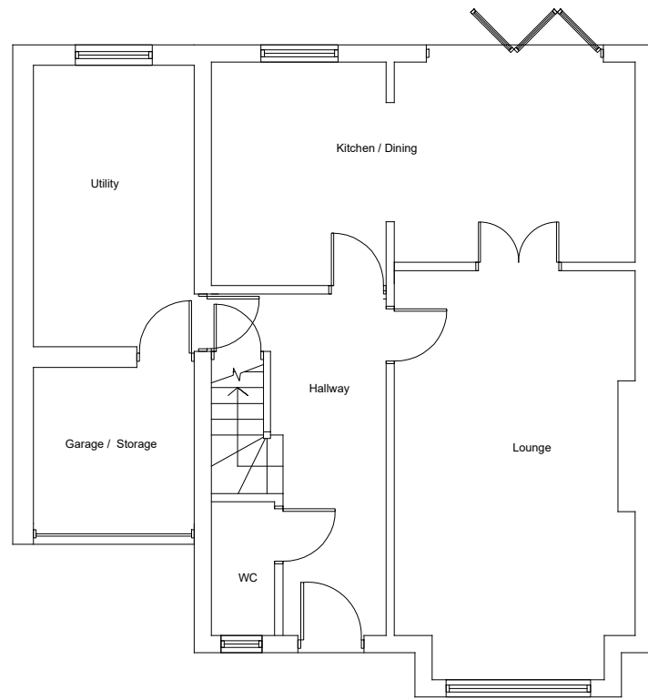
Proposed Ground Floor Plan 1:100
