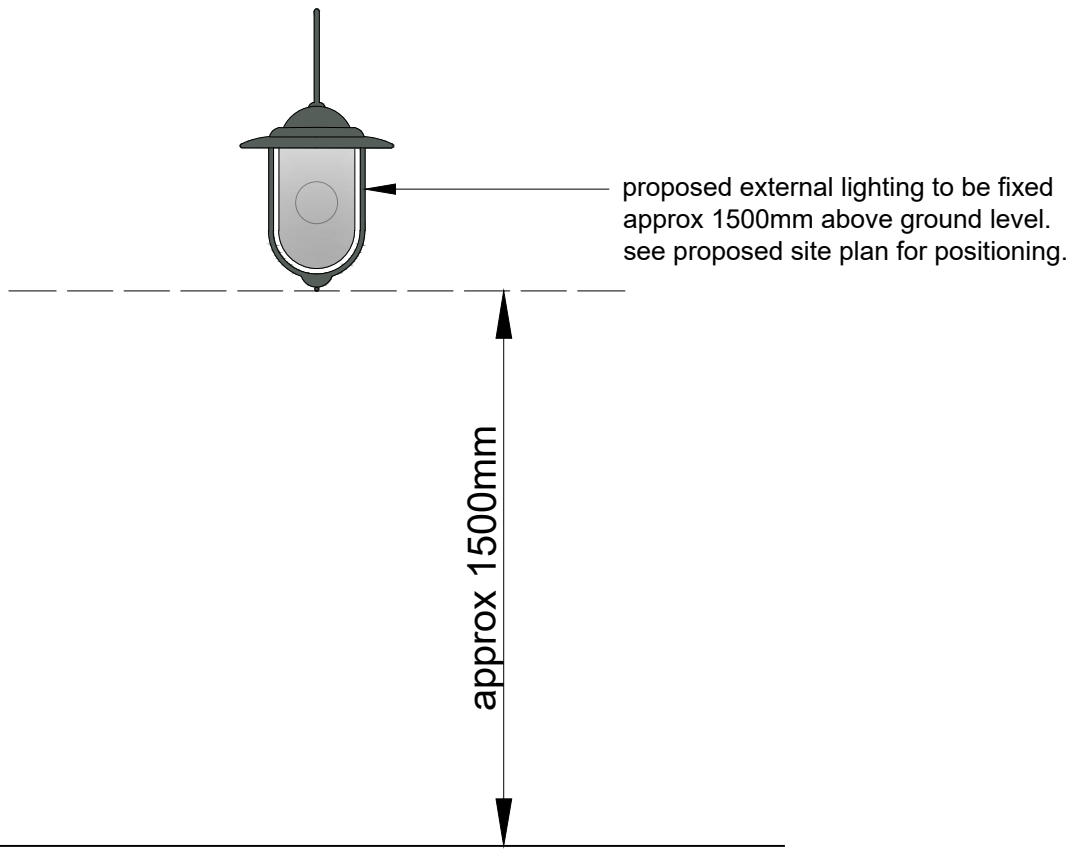
PROPOSED EXTERNAL LIGHTING 1:20 SCALE
