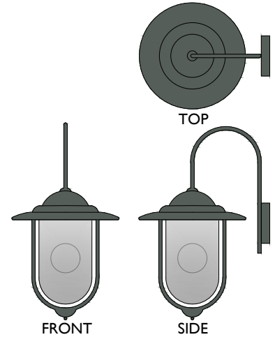
PROPOSED EXTERNAL LIGHTING 1:20 SCALE
