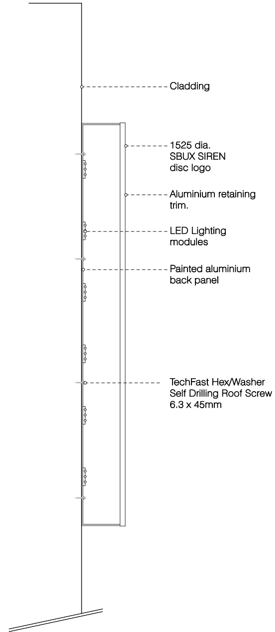
SECTION VIEW OF ROOF BLADE SIGNAGE
