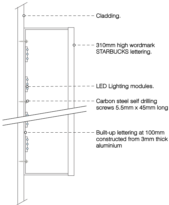
FIXING DETAIL (Section View)
