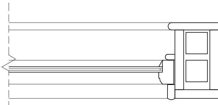
03 Typical SlimLite Double Glazed Plan - Type B Windows 1:5
