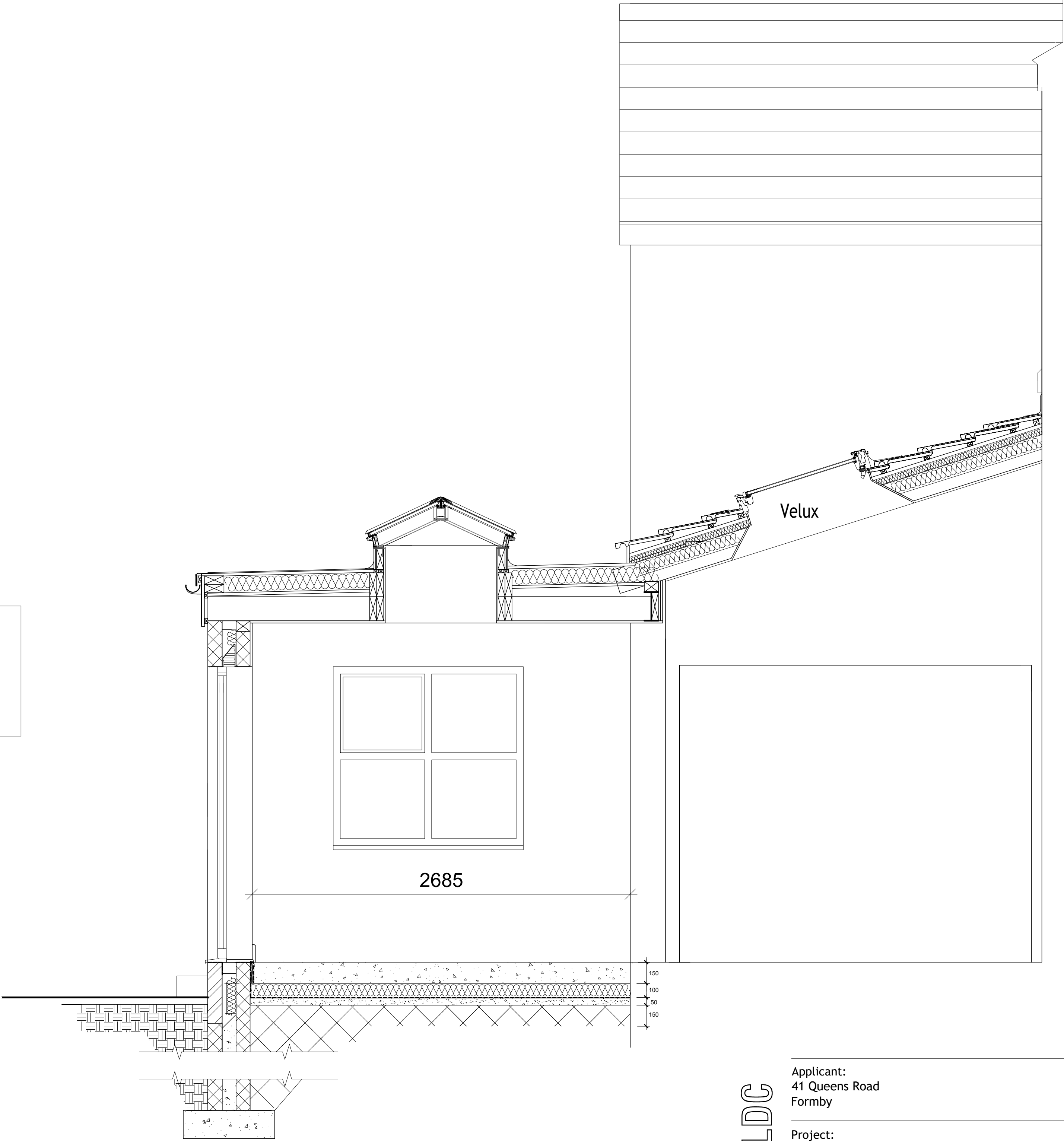
SECTION B - B
