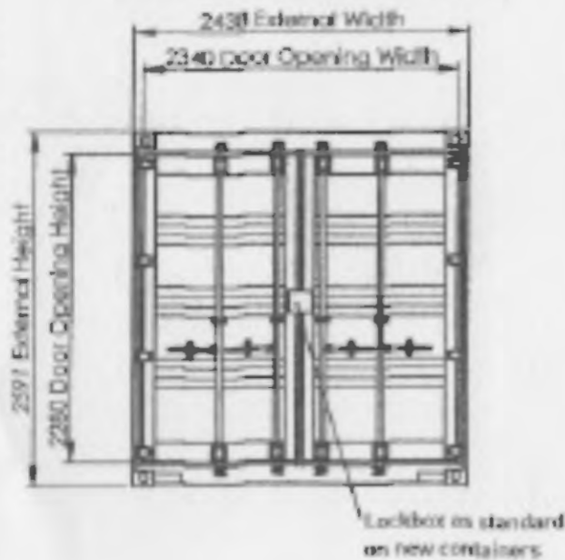
Front End Elevation
