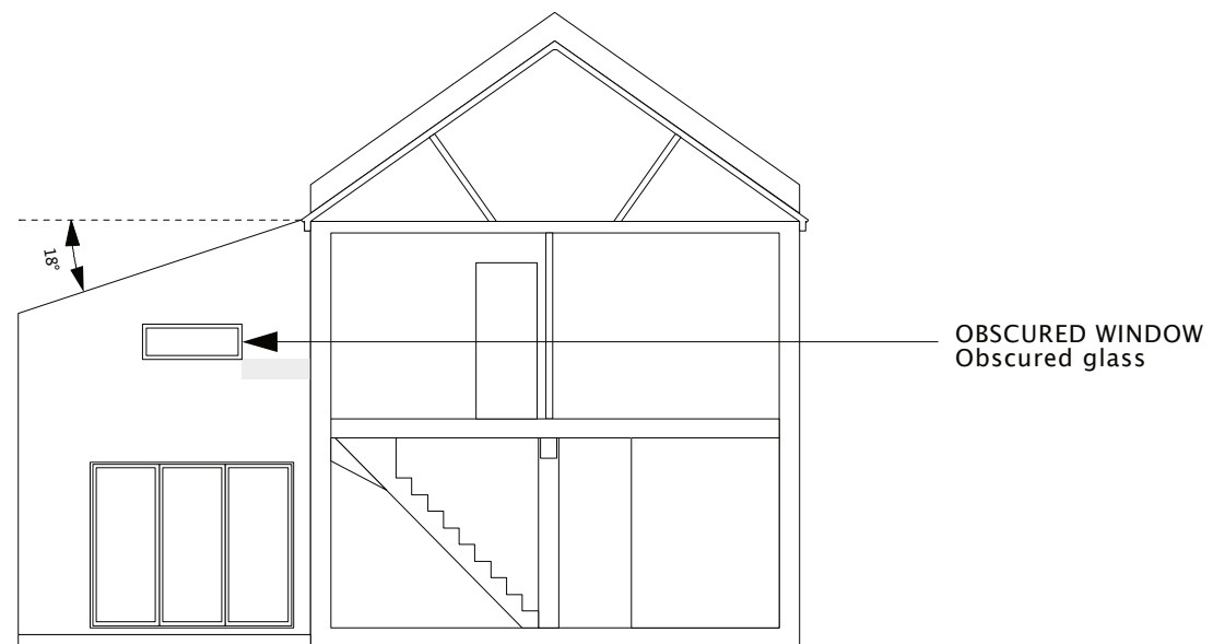
SIDE ELEVATION/SECTION (SOUTH)
