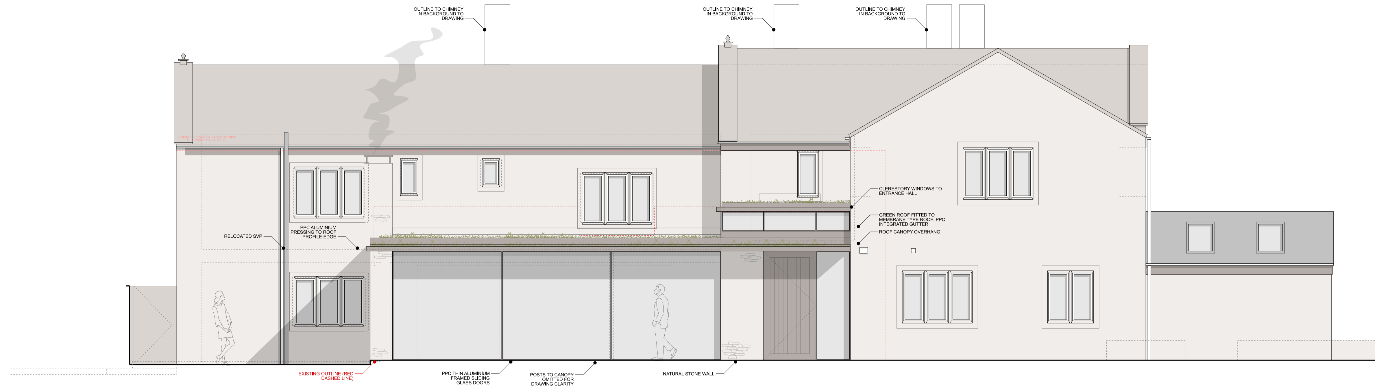
NORTH ELEVATION
