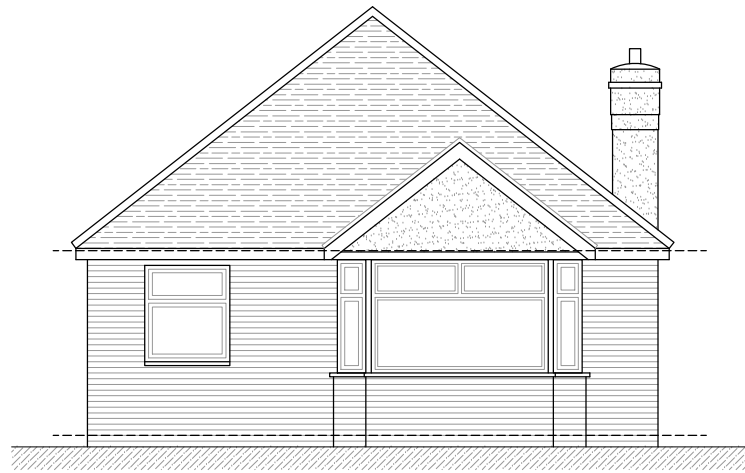
Front (east-facing) Elevation 1:100
