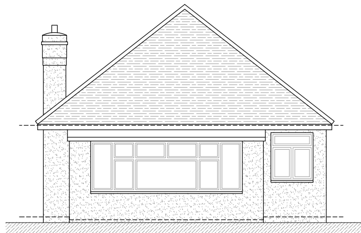
Rear (west-facing) Elevation 1:100
