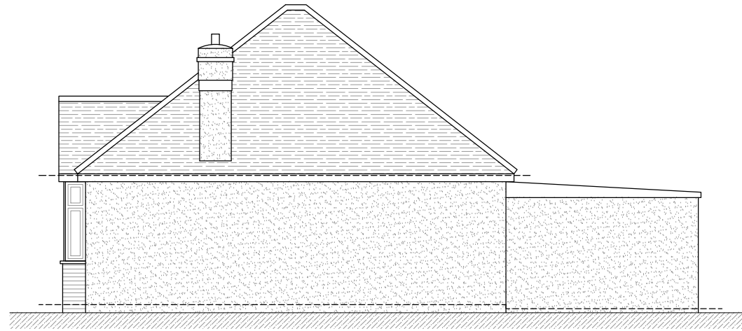
Side (north-facing) Elevation 1:100
