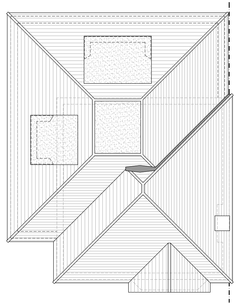
Roof Plan 1:100
