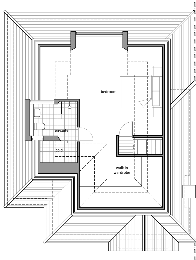
Room-in-Roof Plan 1:100
