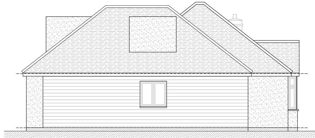
Side (south-facing) Elevation 1:100
