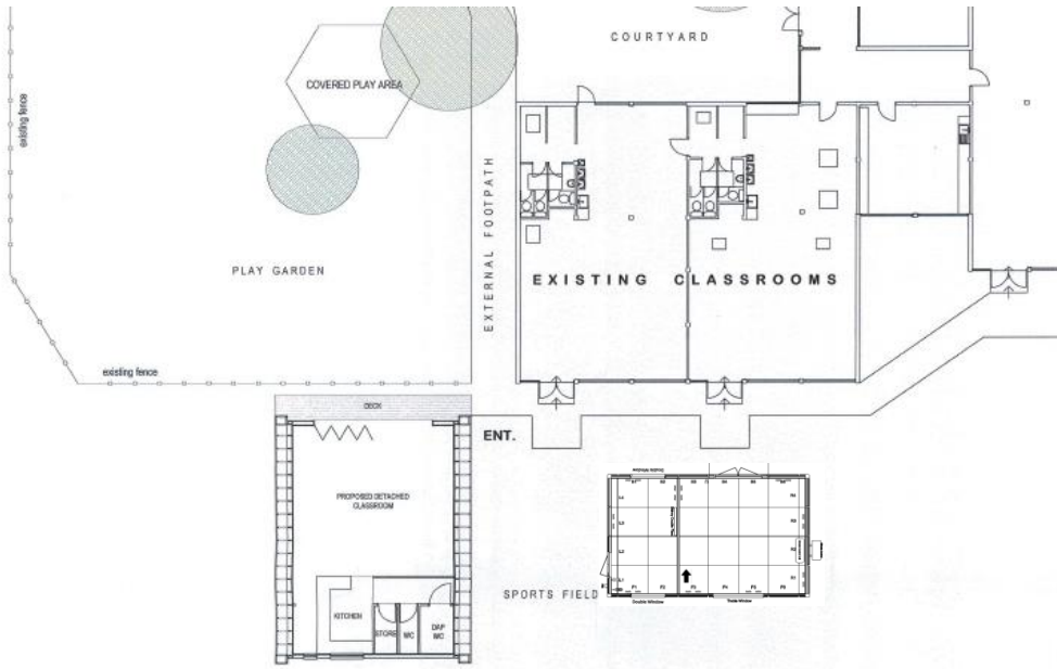
EXISTING PLAN ABOVE, PROPOSED PLAN BELOW
