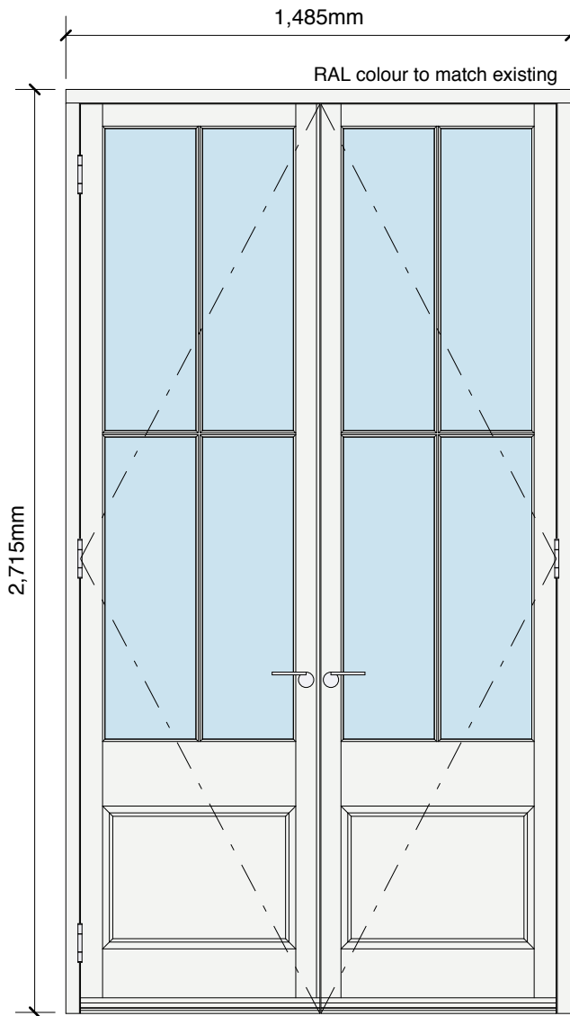
FRENCH DOOR ELEVATION 1:20 @ A4
