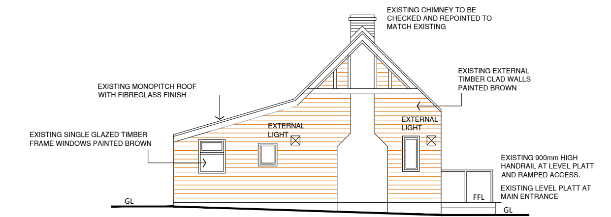
EXISTING SIDE ELEVATION 1:100 SCALE
