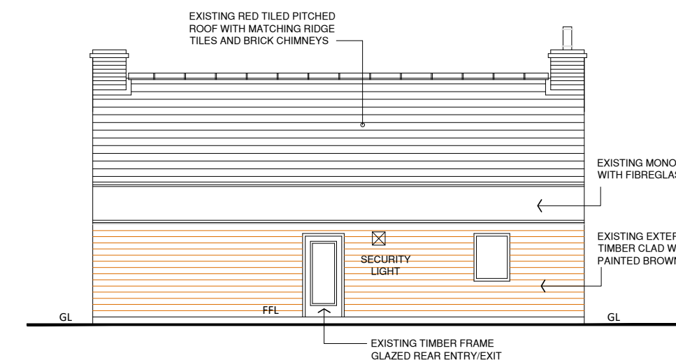
EXISTING REAR ELEVATION 1:100 SCALE
