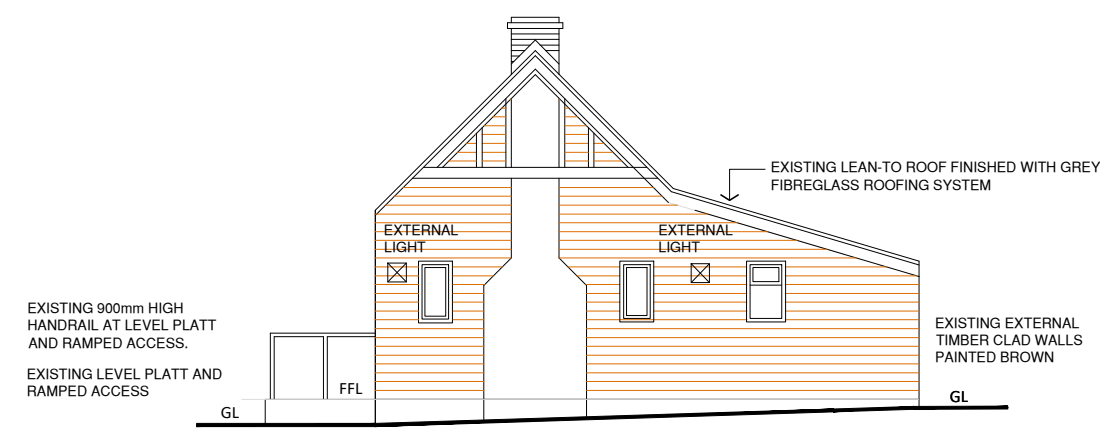
EXISTING SIDE ELEVATION 1:100 SCALE
