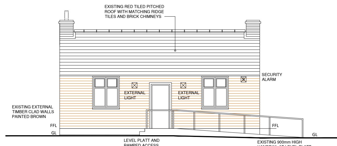
EXISTING FRONT ELEVATION 1:100 SCALE
