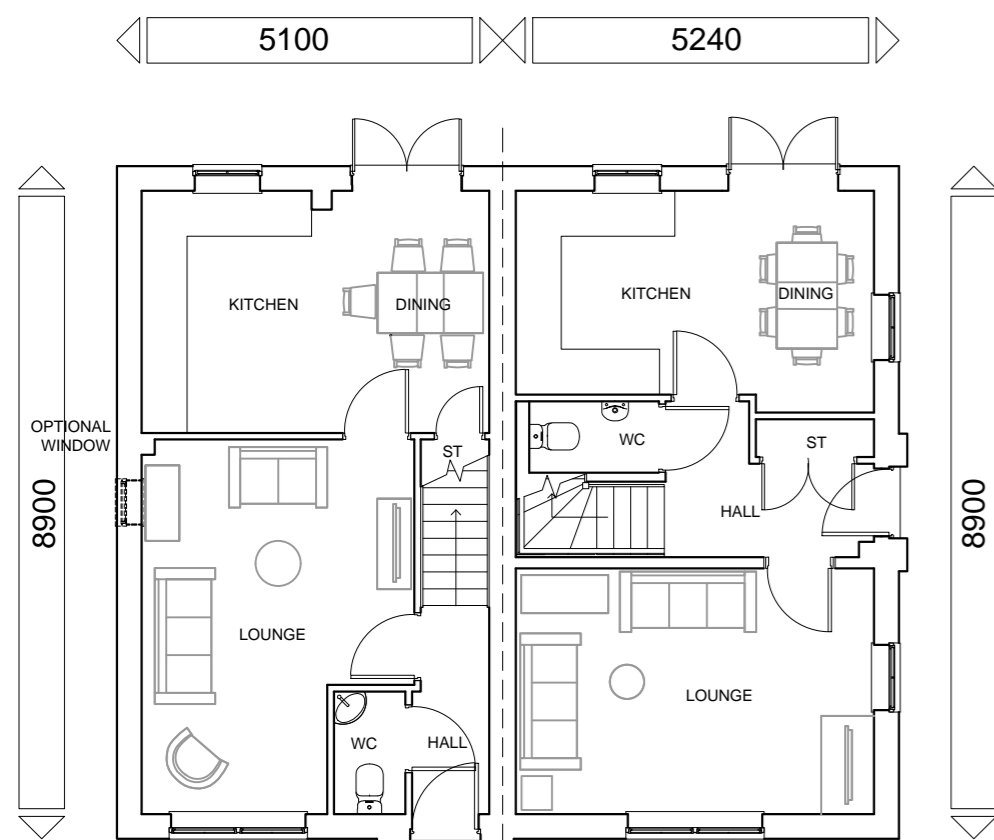
GROUND FLOOR PLAN MAIDSTONE MORESBY
