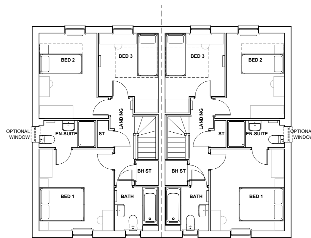
FIRST FLOOR MAIDSTONE (X) MAIDSTONE (X)
