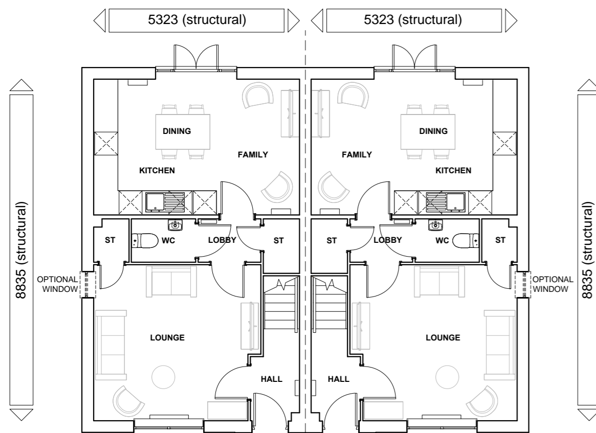
GROUND FLOOR MAIDSTONE (X) MAIDSTONE (X)
