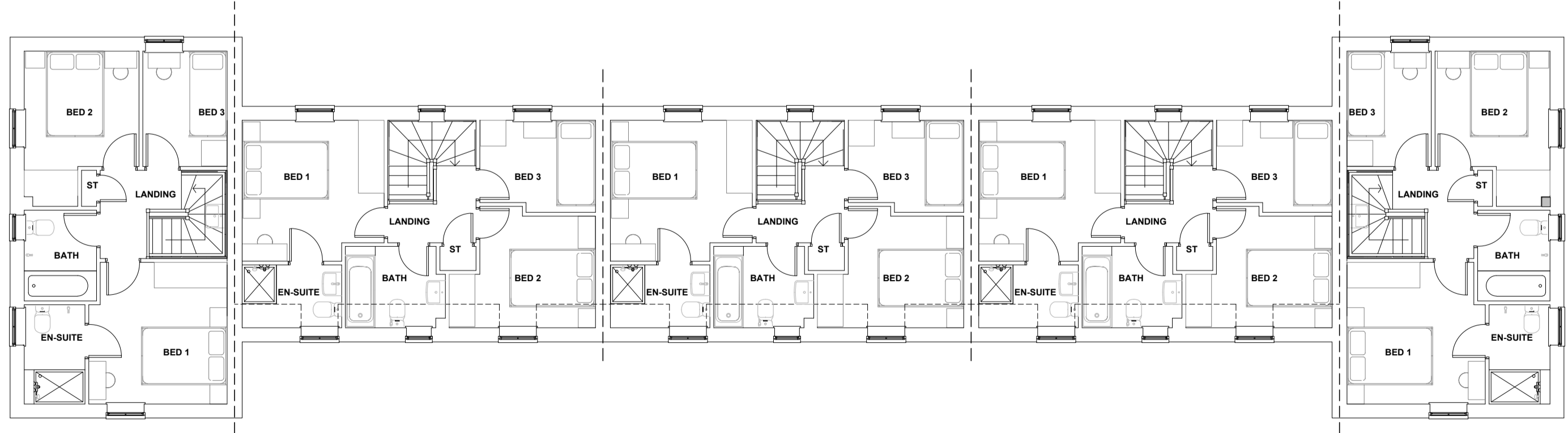
FIRST FLOOR Moresby (SP) Buchanan (SP) Buchanan (SP) Buchanan (SP) Moresby (SP)
