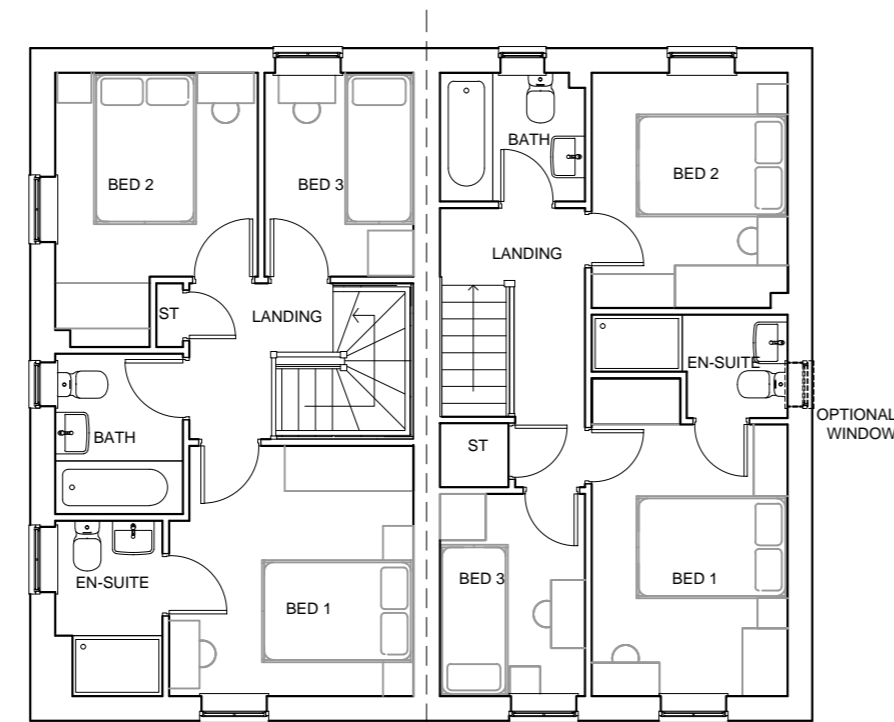
FIRST FLOOR PLAN MORESBY MAIDSTONE
