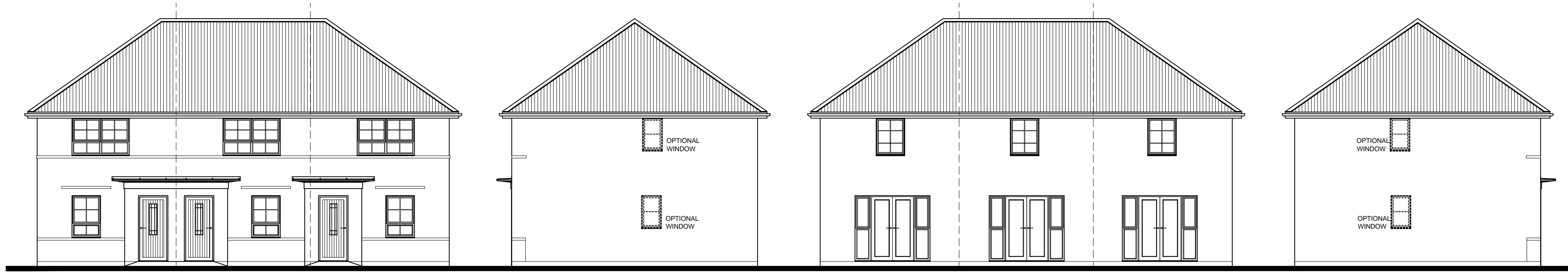
FRONT ELEVATION
