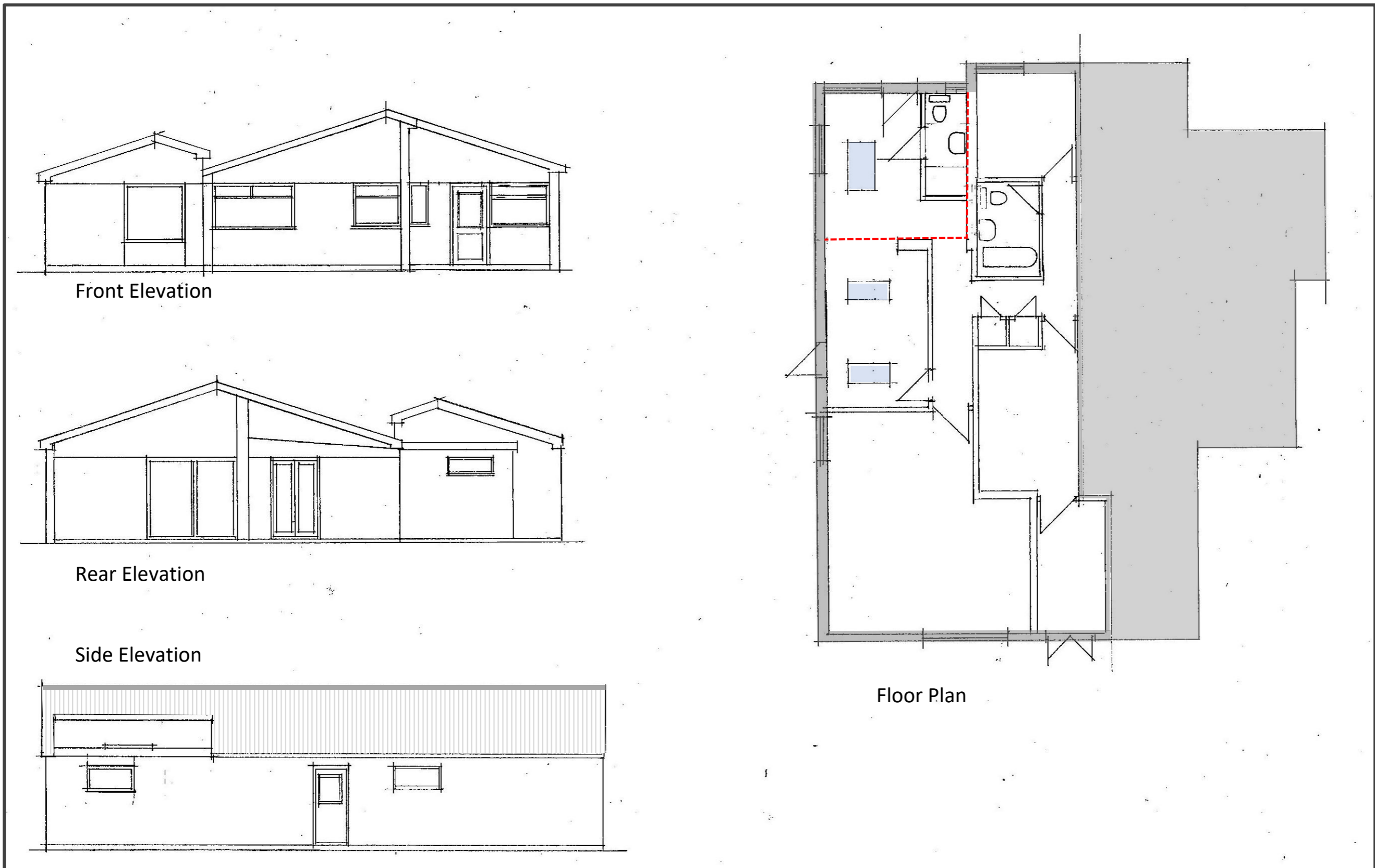
53 Sandhurst Road, Proposed Extension Proposed Plan and Elevations, Scale 1:100 @ A3
