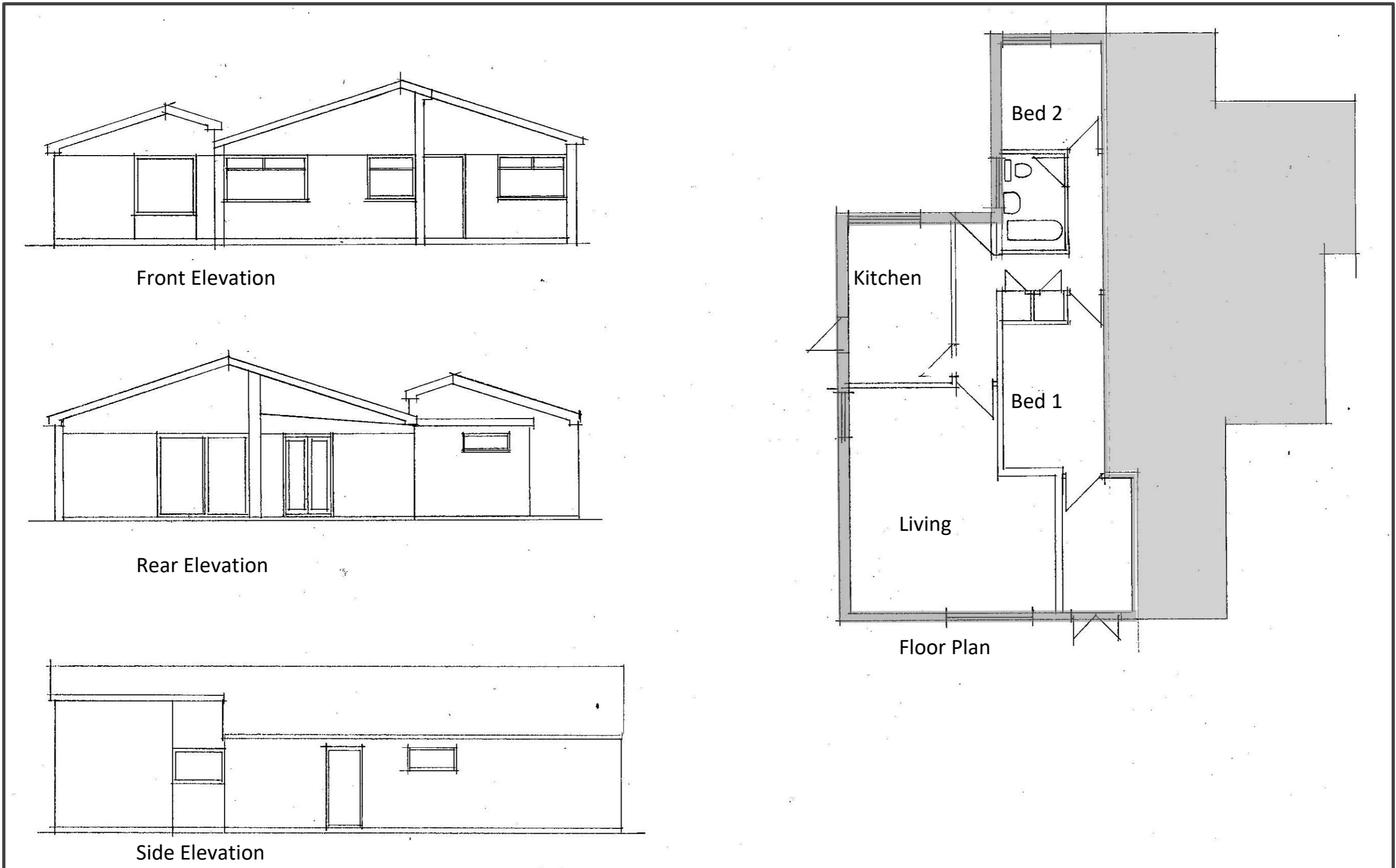
53 Sandhurst Road, Proposed Extension Existing Plan and Elevations, Scale 1:100 @ A3
