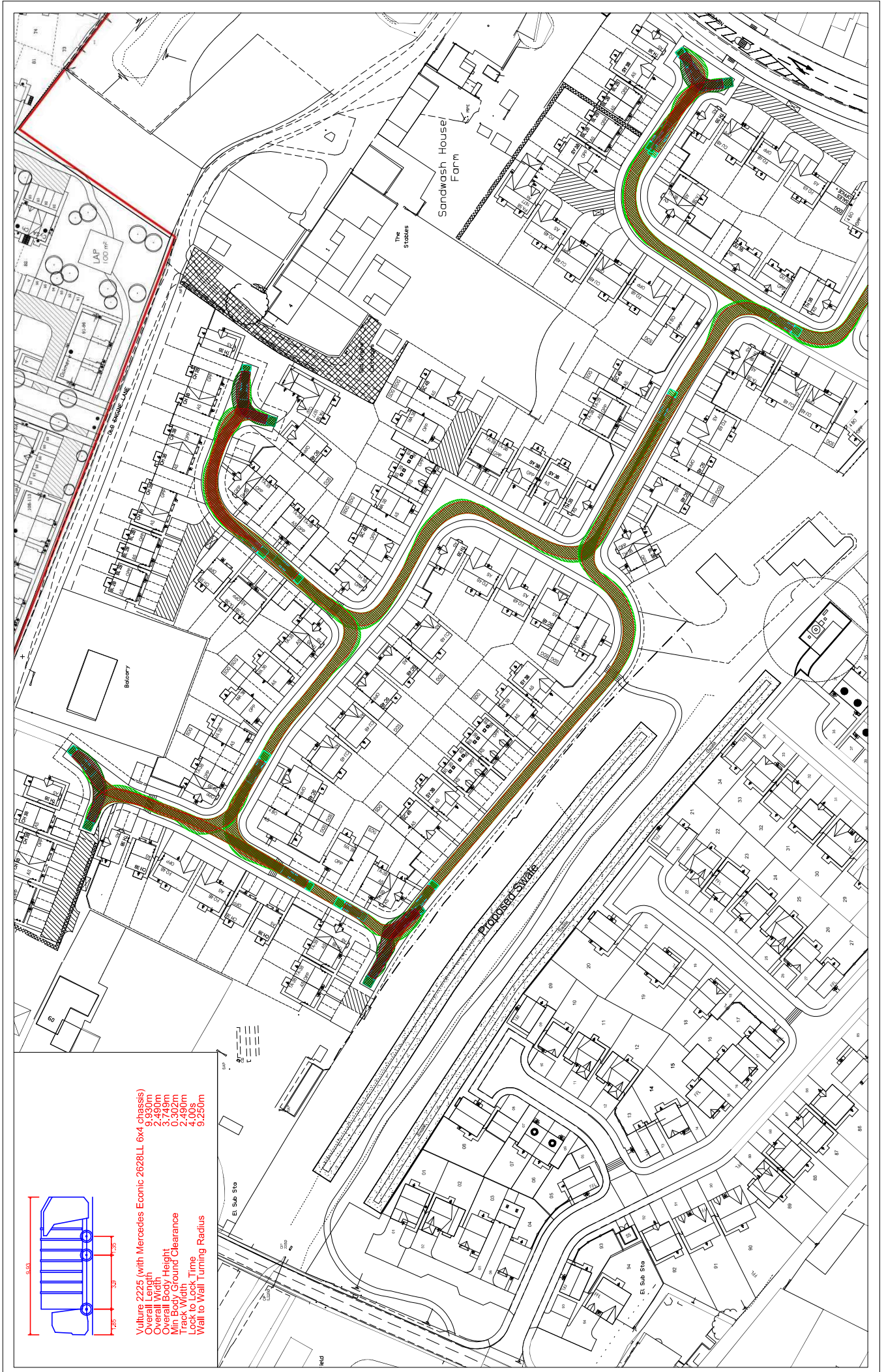
Figure 5.3 Sweep Path Analysis: Large Refuse Vehicle Passing Through Site (Northern Section) (1:1,000 @ A3)
