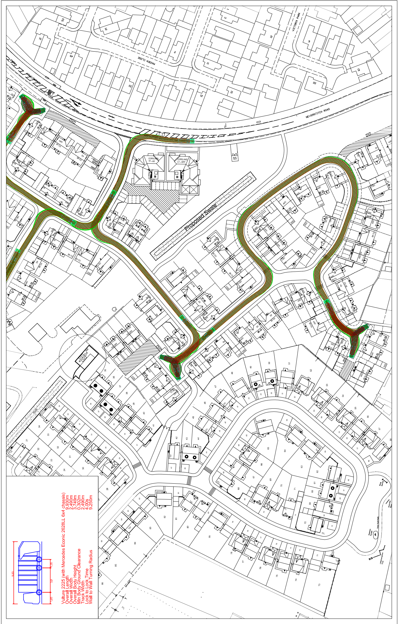
Figure 5.4 Sweep Path Analysis: Large Refuse Vehicle Passing Through Site (Southern Section) (1:1,000 @ A3)
