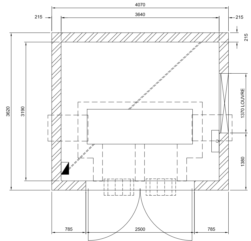
FLOOR PLAN
