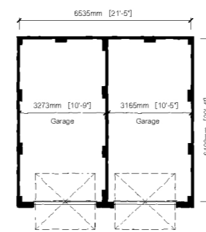
Plan Variation - 1:200
