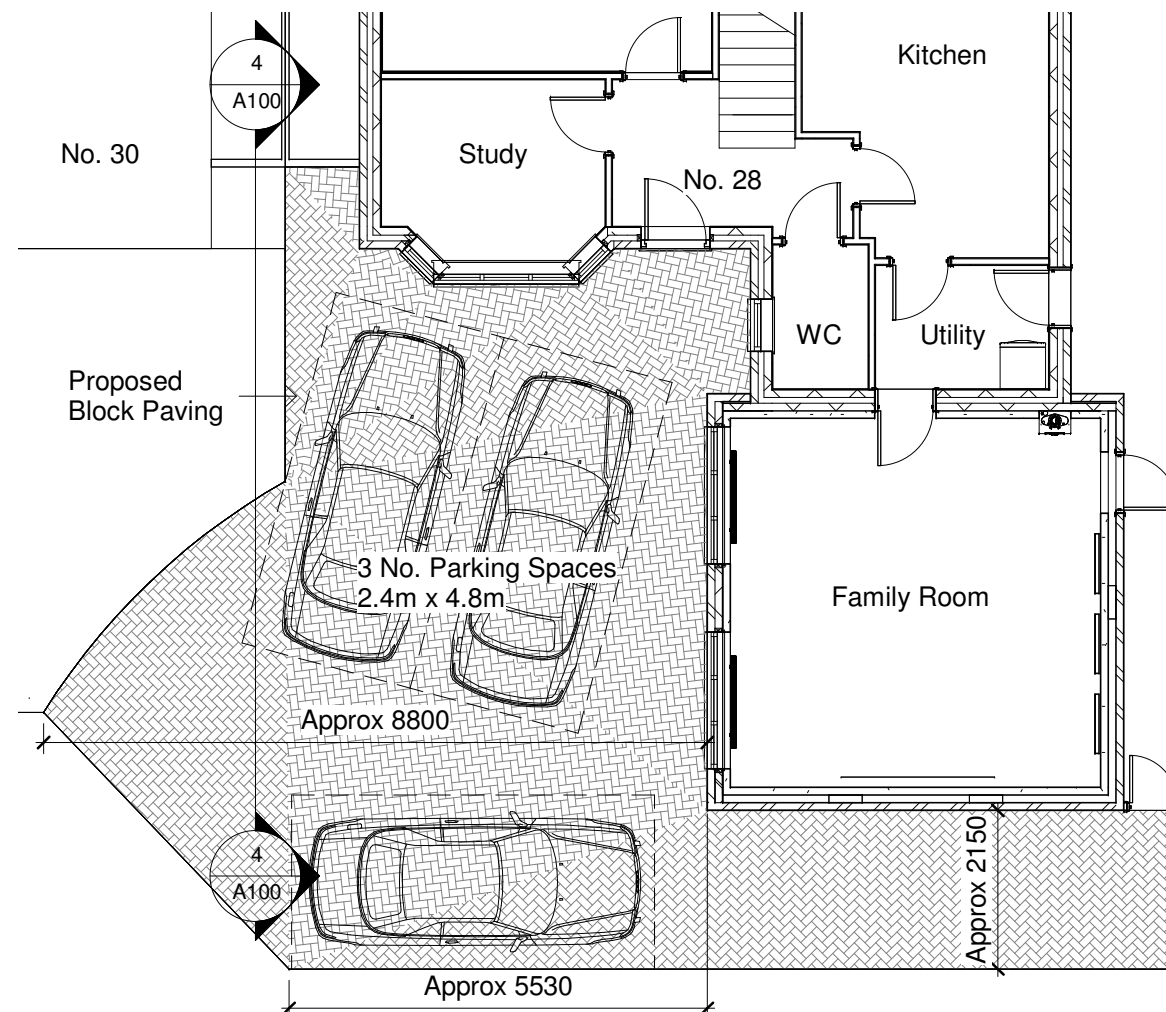
2 Proposed Plan 1 : 100
