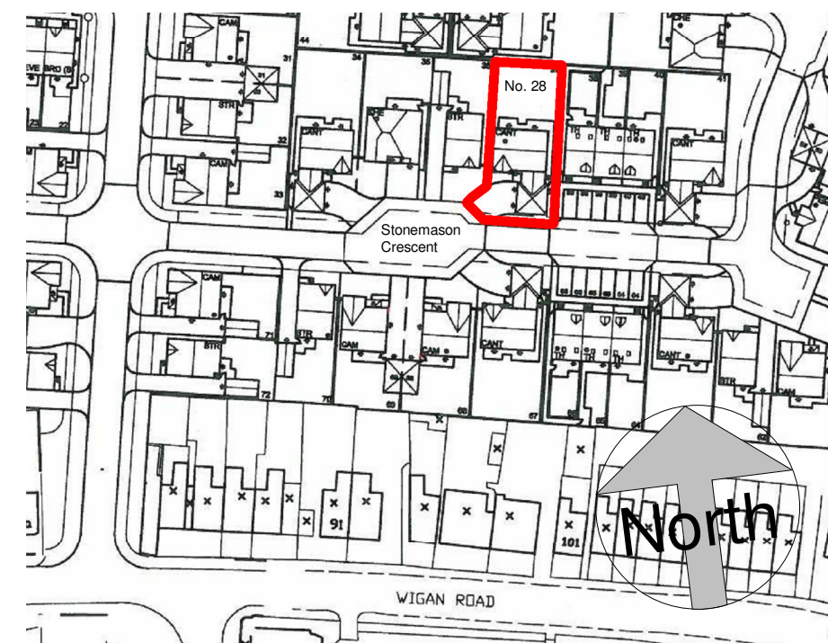
5 Location Plan 1 : 1250
