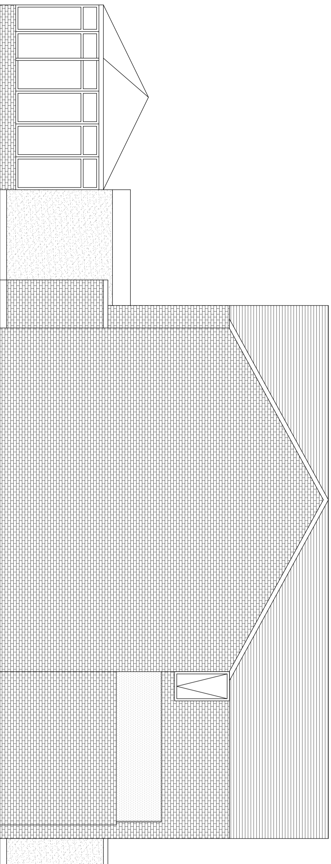
PROPOSED SIDE ELEVATION LAYOUT 1 (SCALE 1:50)
