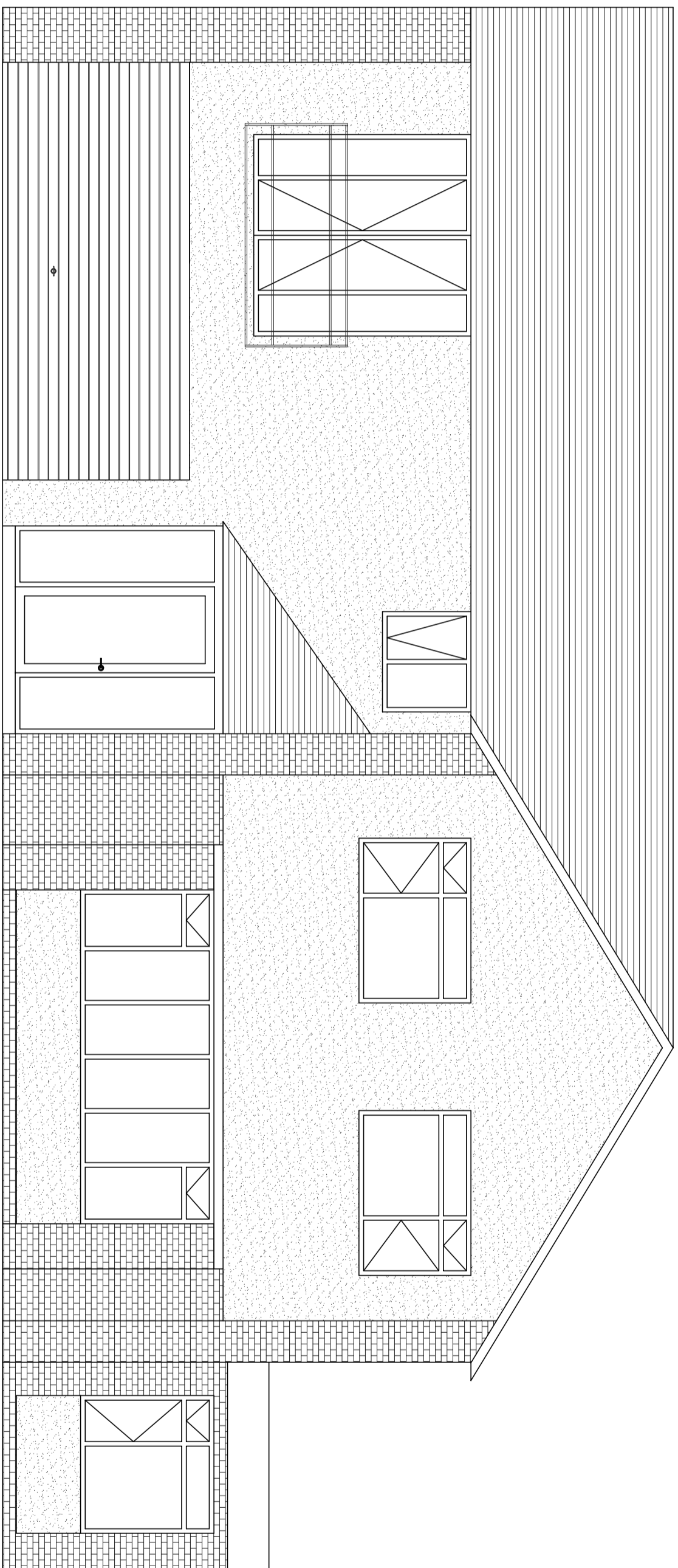
EXISTING FRONT ELEVATION LAYOUT (SCALE 1:50)
