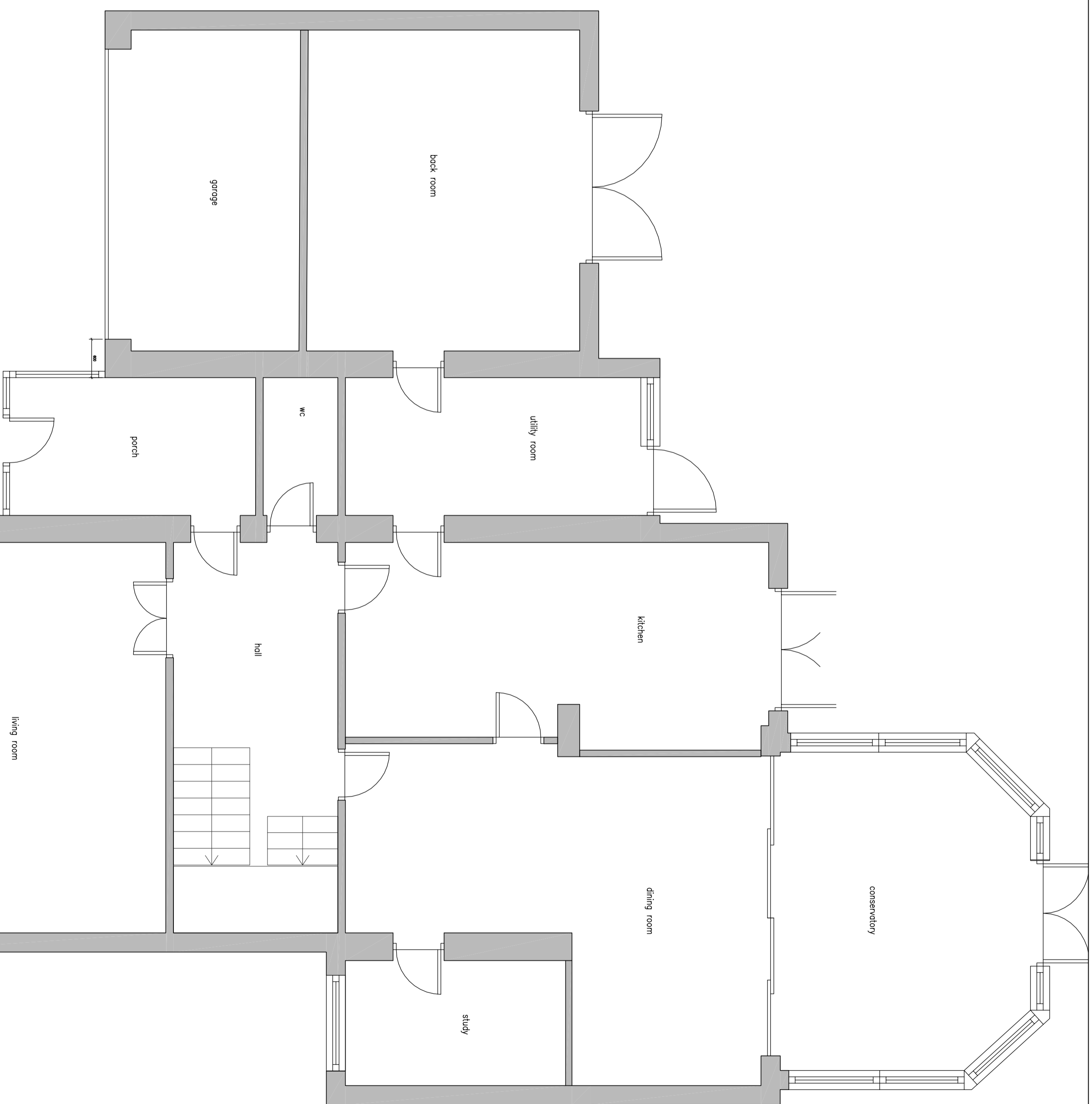
EXISTING GROUND FLOOR LAYOUT (SCALE 1:50)
