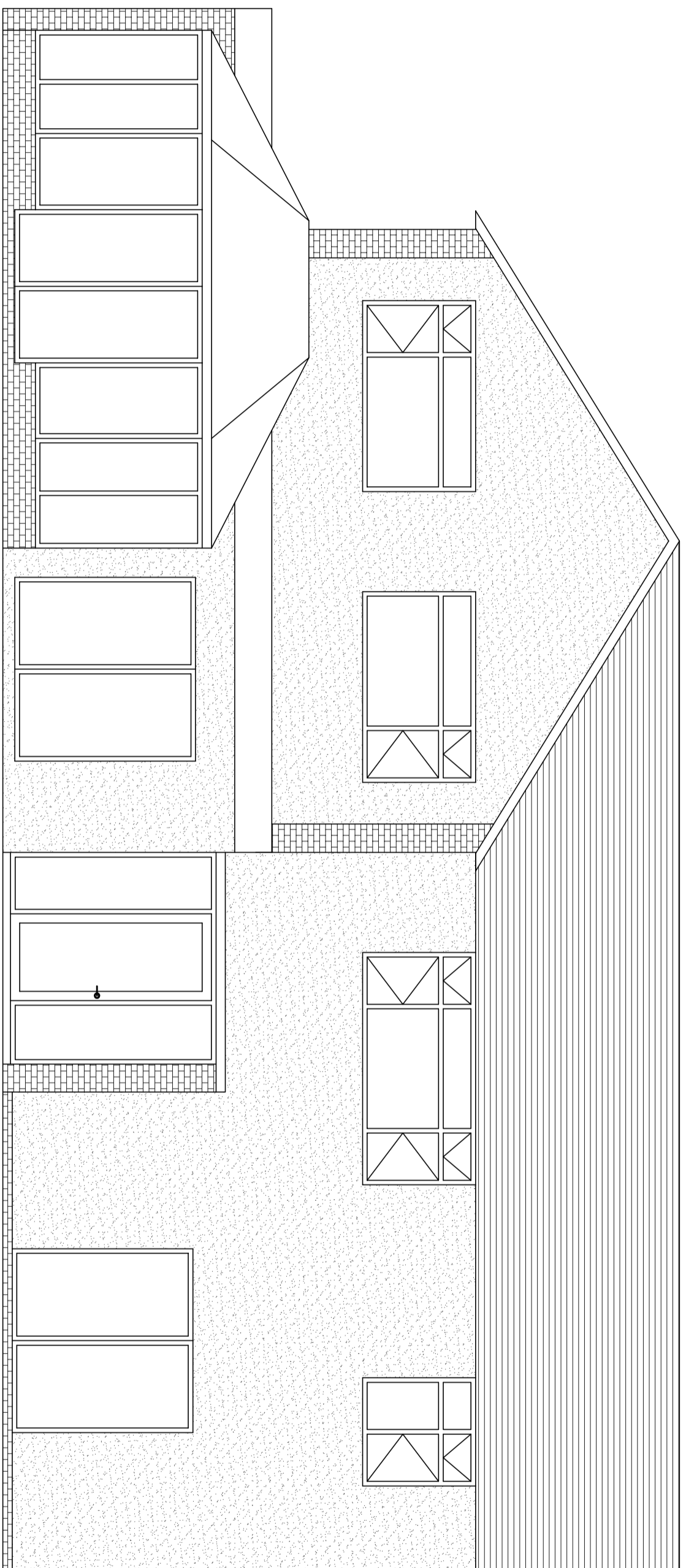
PROPOSED REAR ELEVATION LAYOUT (SCALE 1:50)
