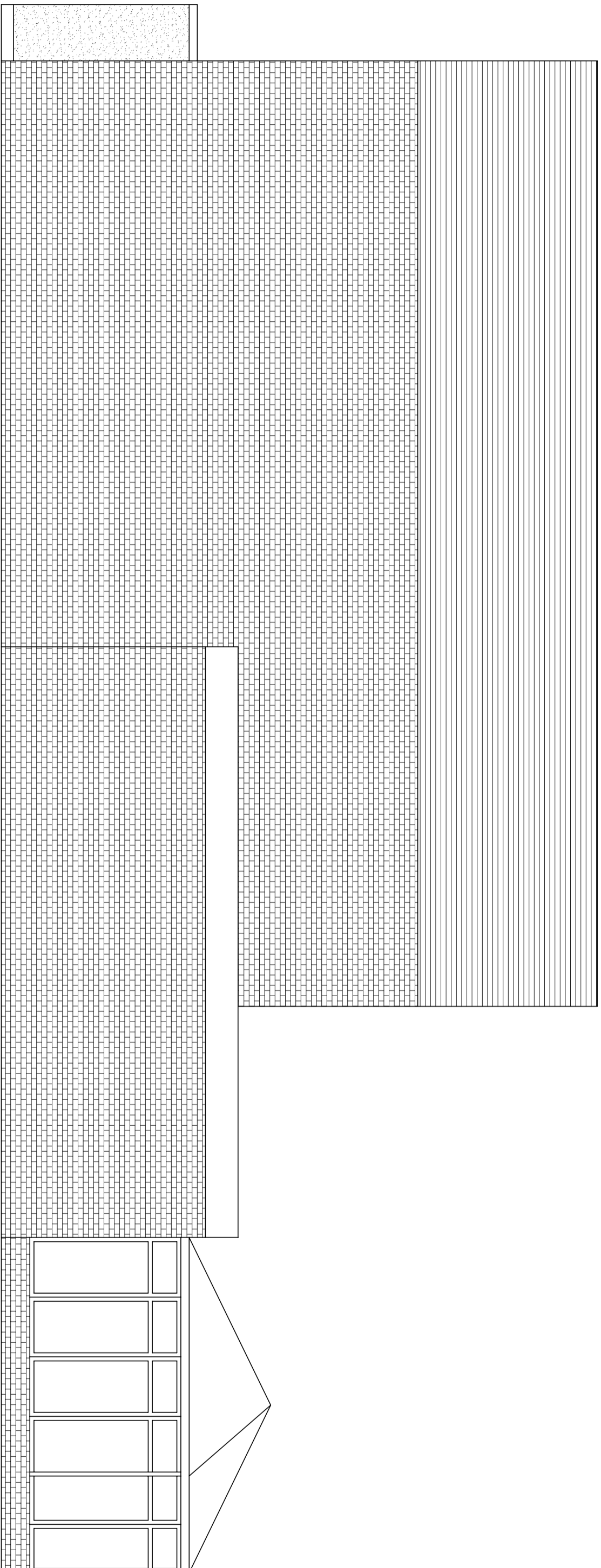
PROPOSED SIDE ELEVATION LAYOUT 2 (SCALE 1:50)
