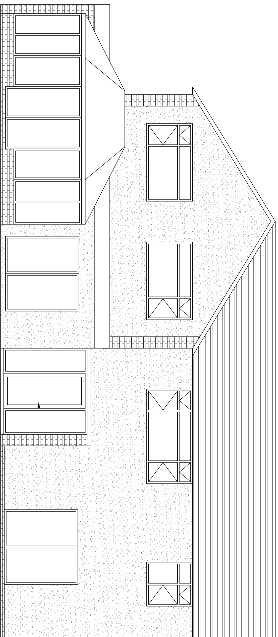
EXISTING REAR ELEVATION LAYOUT (SCALE 1:50)
