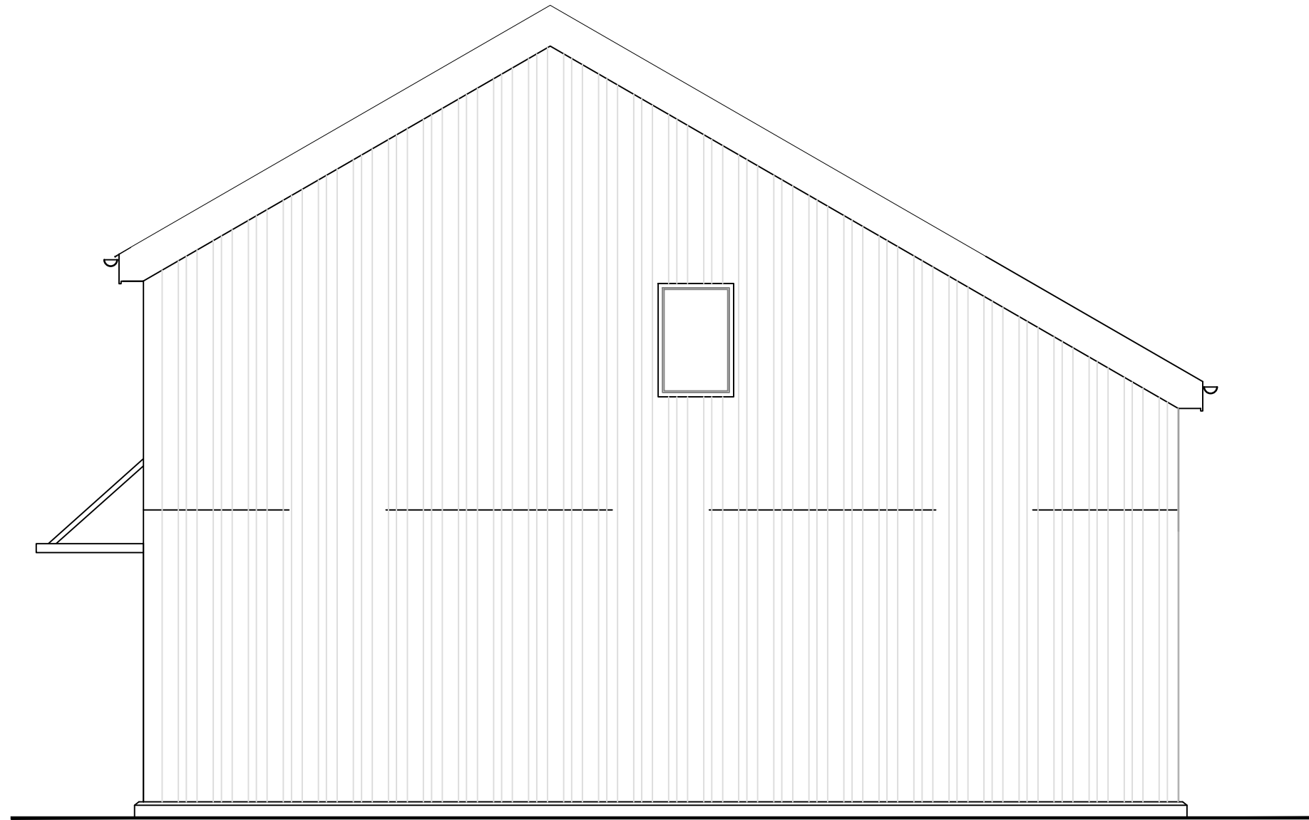
ELEVATION TO EAST
