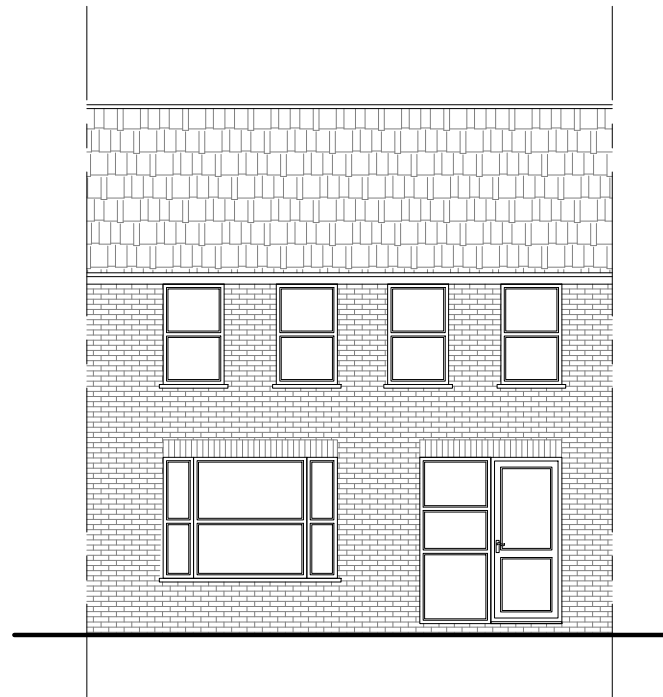
Rear Elevation
