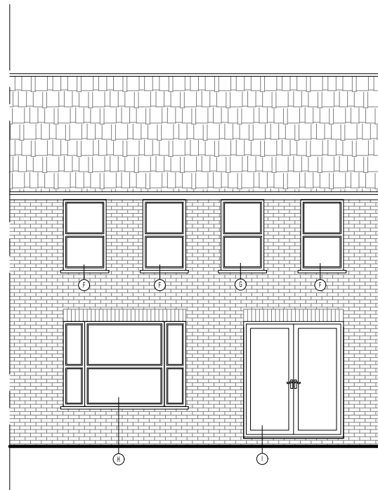
Rear Elevation
