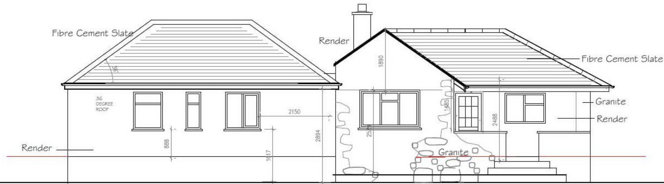
EXISTING SOUTH EAST ELEVATION
