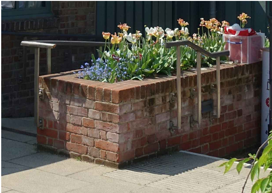
02 Brick planter with stainless steel handrail and planting to match existing
