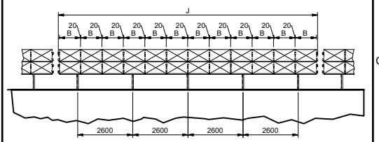
DETAIL MOUNTING SYSTEM - FRONT VIEW SCALE 1:250
