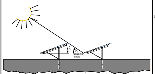
DETAIL MOUNTING SYSTEM - SIDE VIEW SCALE 1:250
