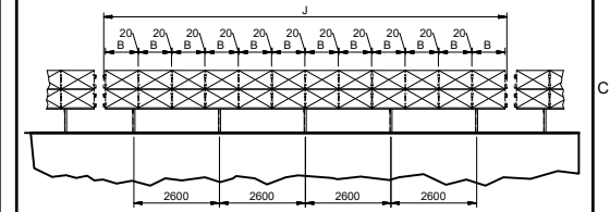
DETAIL MOUNTING SYSTEM - FRONT VIEW SCALE 1:250
