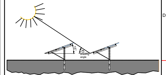
DETAIL MOUNTING SYSTEM - SIDE VIEW SCALE 1:250
