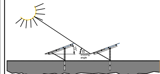
DETAIL MOUNTING SYSTEM - SIDE VIEW SCALE 1:250
