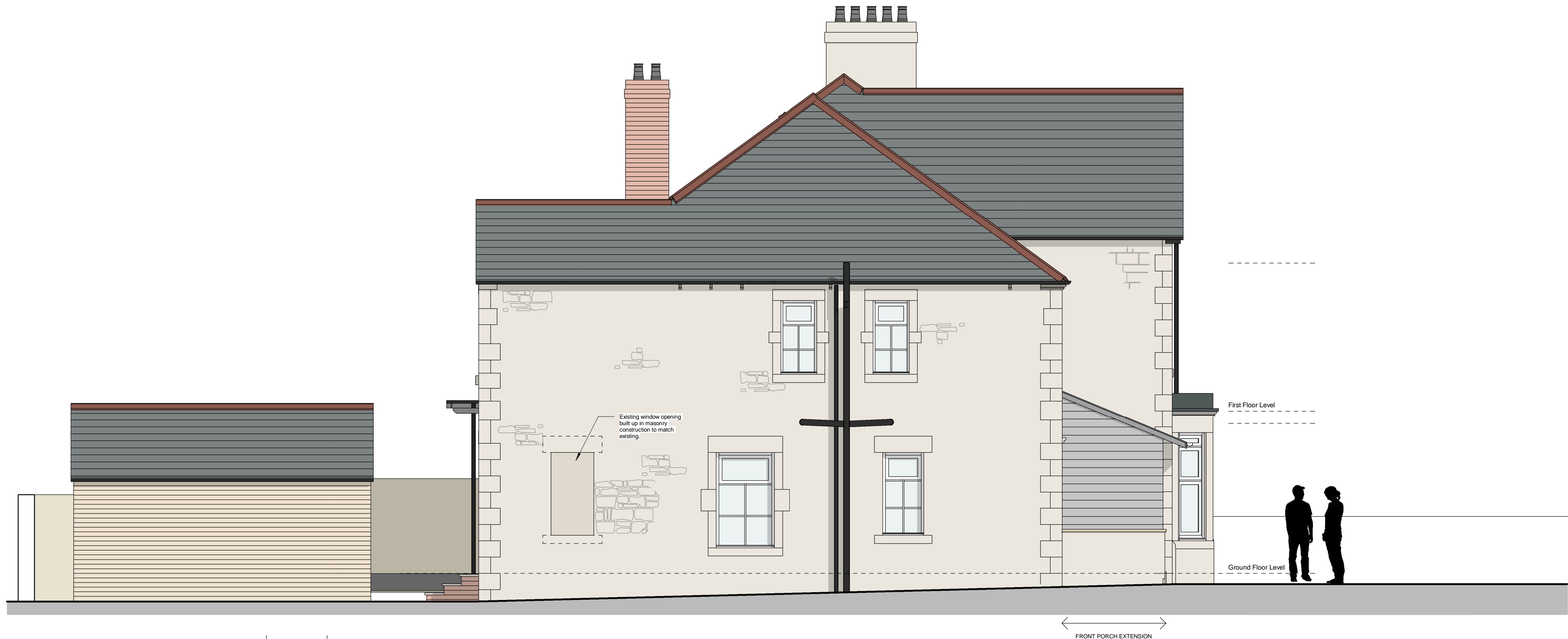
PROPOSED NORTH (SIDE) ELEVATION
