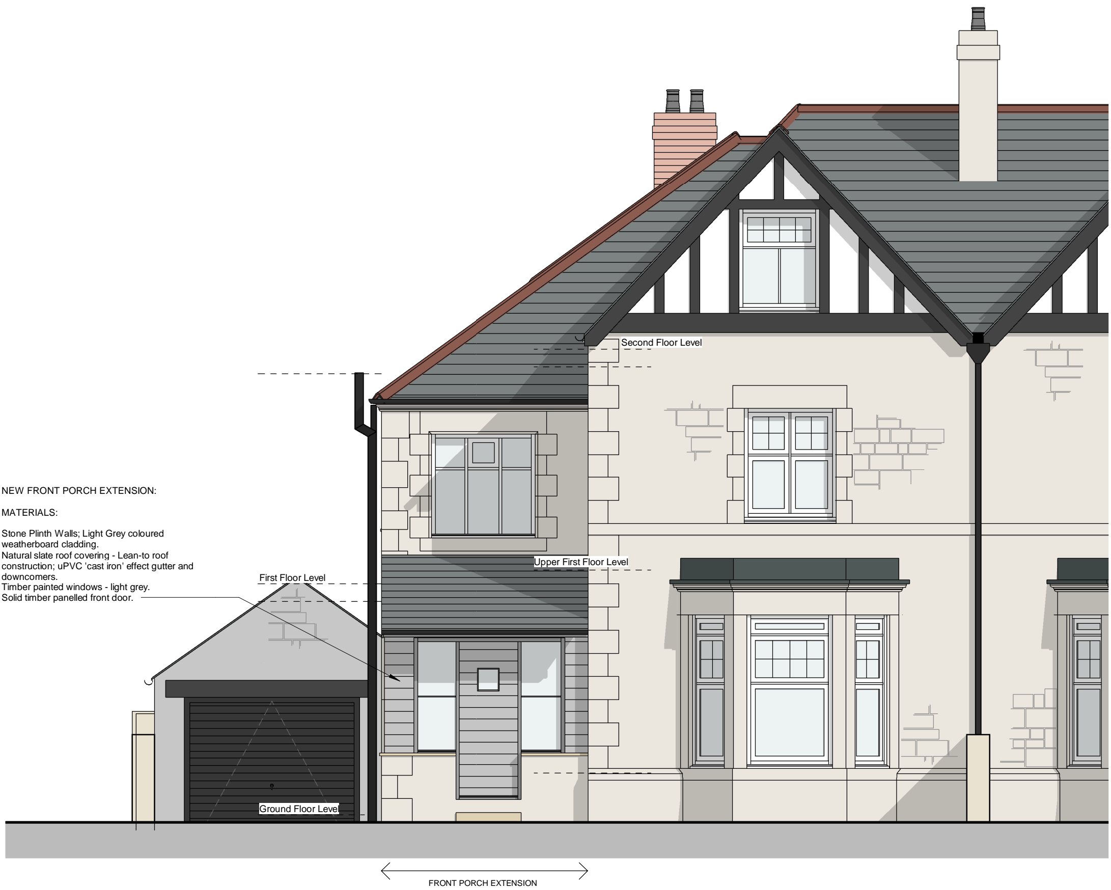
PROPOSED WEST (FRONT) ELEVATION
