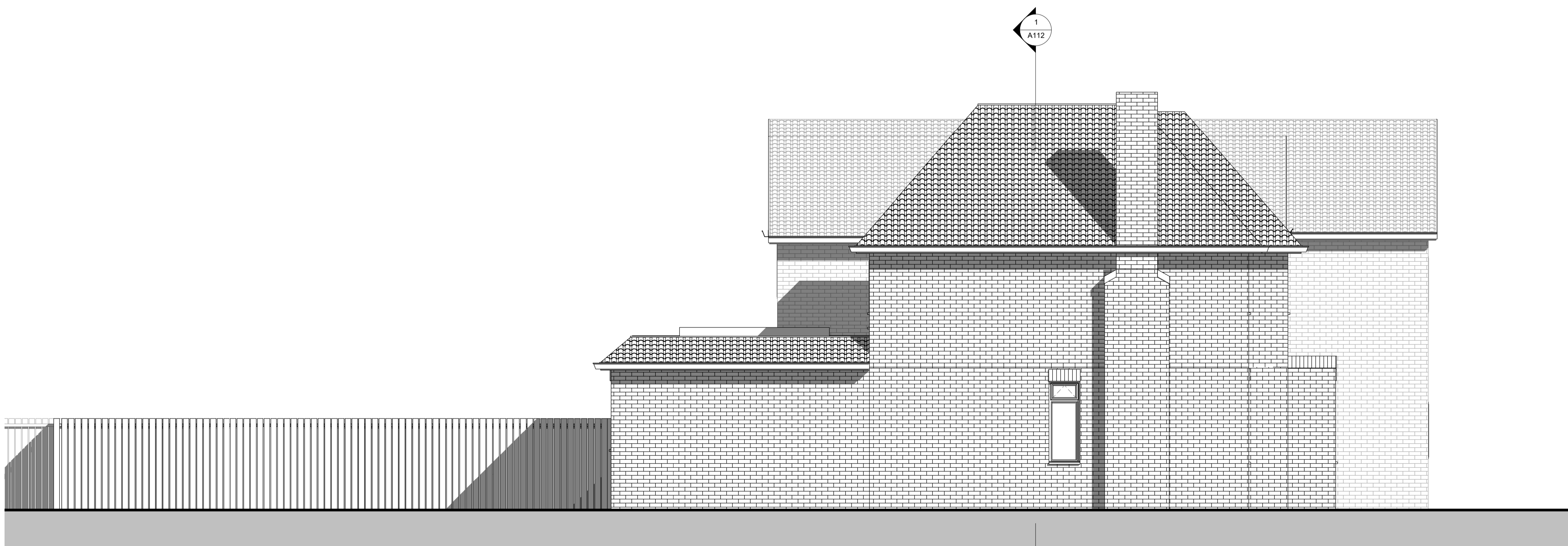
2 Proposed N-W Elevation 1 : 50
