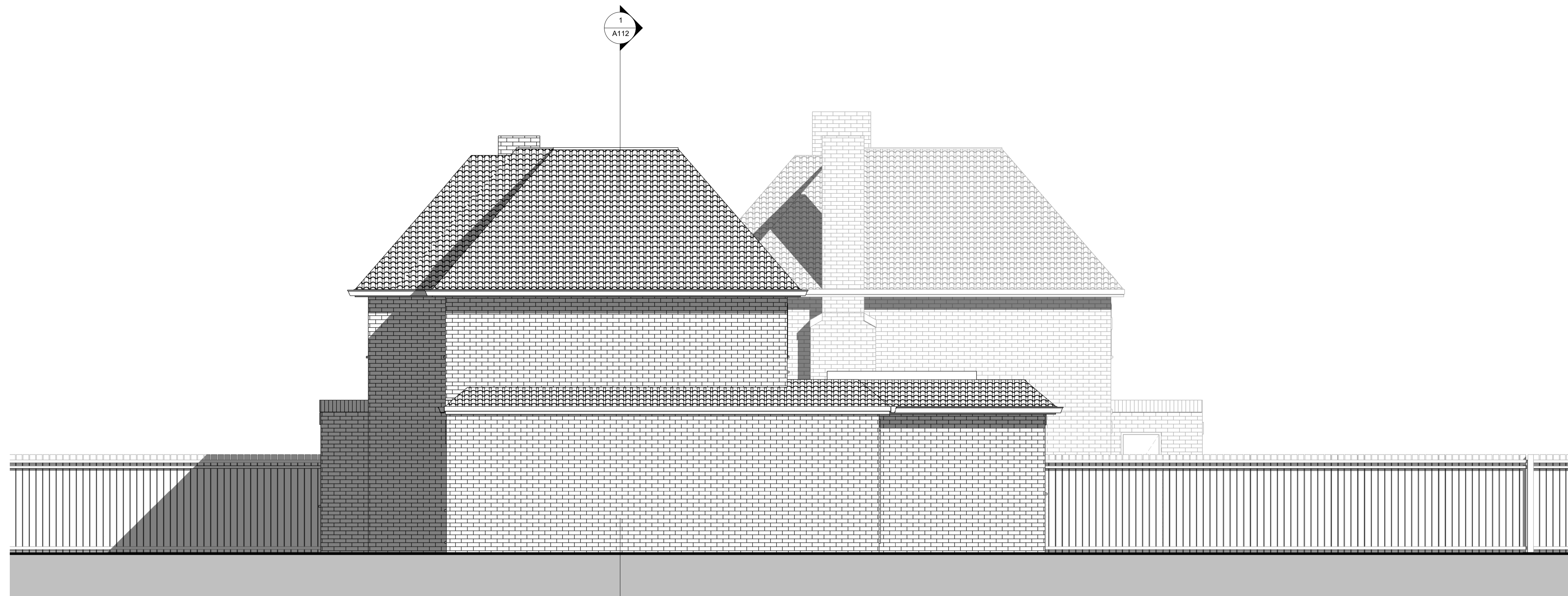
1 Proposed S-E Elevation 1 : 50
