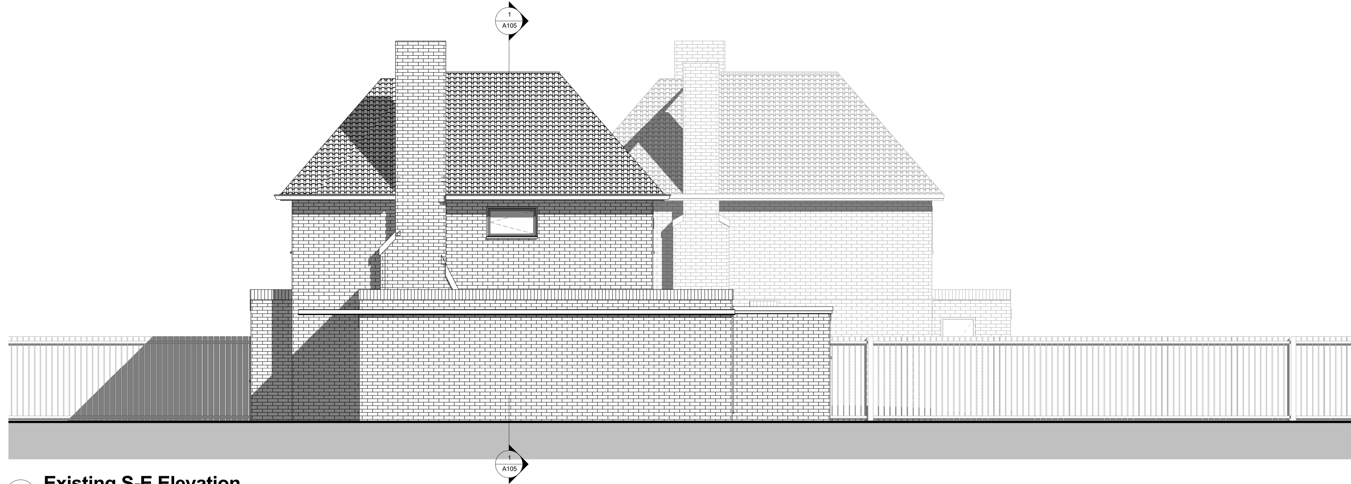
1 Existing S-E Elevation 1 : 50
